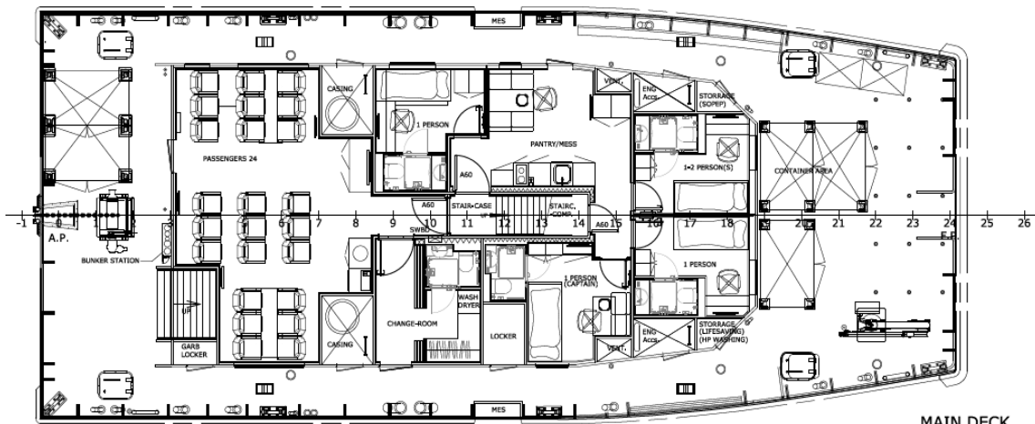
MAIN DECK
