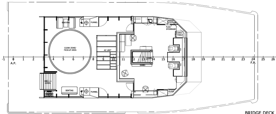
BRIDGE DECK
