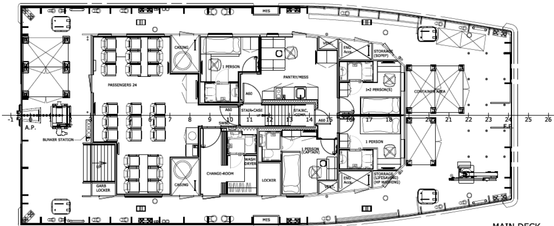
MAIN DECK
