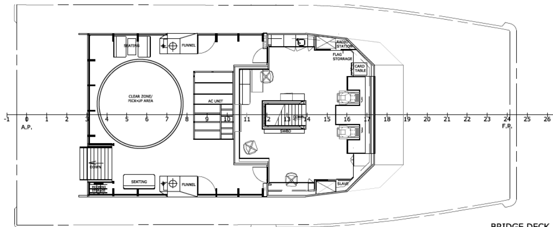
BRIDGE DECK
