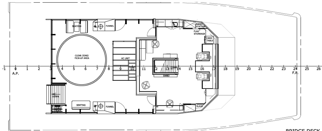
BRIDGE DECK
